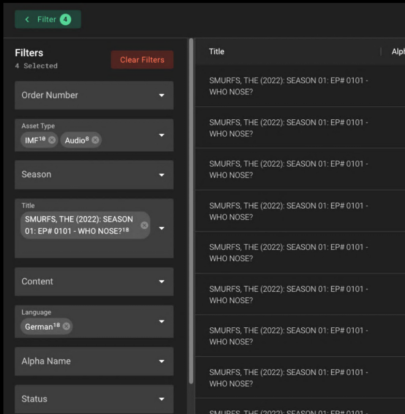
Fig. 3 – Asset Dashboard – Filter drawer with values selected on various filters.
